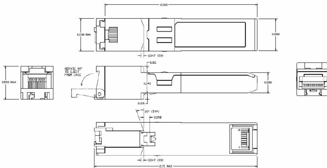
Figure 2. QT-SFP-T mechanical dimensions
